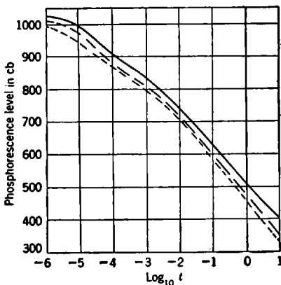
FIG. 18-25.—Phosphorescent decay following single pulse excitation and current density of j = 4 \text{ ma/cm}^2 . Time t in seconds. Excitation period 30 \mu\text{sec} ---; 50 \mu\text{sec} - · - · -; 200 \mu\text{sec} —. Screen type: (88)ZnS: (12)-CdS:Cu.
